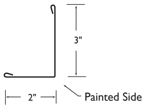
3 2 x 3 Eave Flashing
