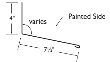
2 Endwall Flashing
