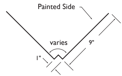
4 W-Valley
