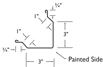
5 3 x 3 Outside Corner
