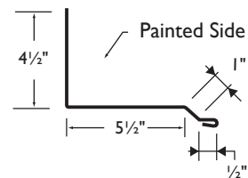
6 Sidewall Flashing
