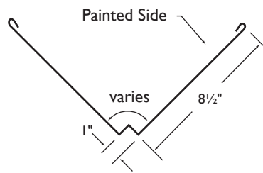
4 Open Hem W-Valley
