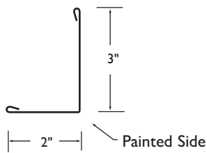
3 2 x 3 Eave Flashing
