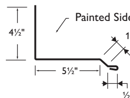
6 Sidewall Flashing
