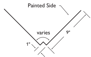
4 W-Valley
