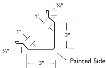
5 3 x 3 Outside Corner
