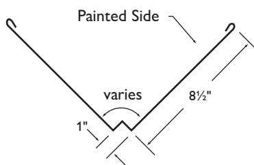
4 Open Hem W-Valley
