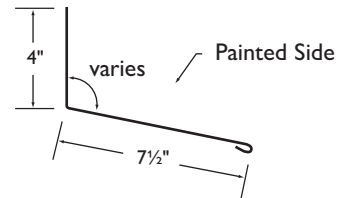
2 Endwall Flashing
